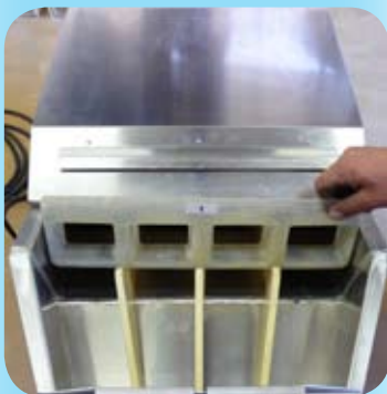
Fish counter with open cover (View on the polyester separation)
