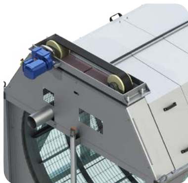
Simple and robust drum driving system.
